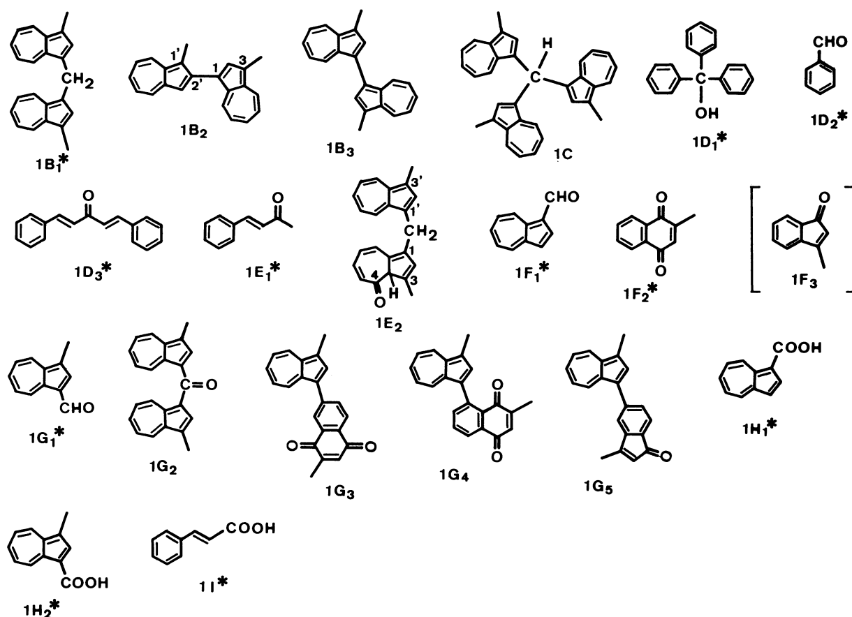
Chart 1. Structures of the autooxidation products from 1 ; *previously known compounds.
